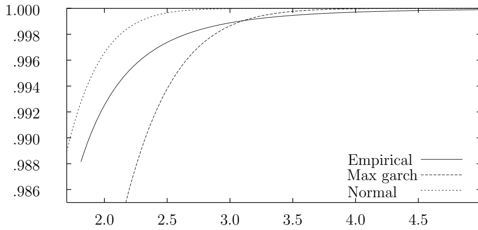
Figure 4: Disribution of SP-500 returns 1990-1996 and Highest GARCH Prediction.
