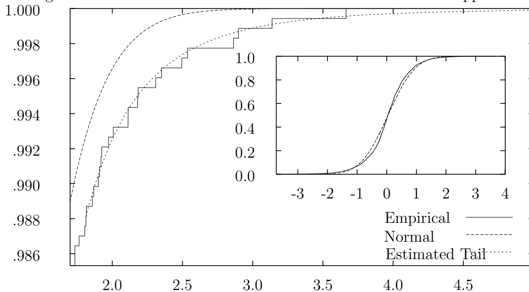
Figure 3: Distribution of SP-500 returns 1990-1996 with fitted upper tail.
